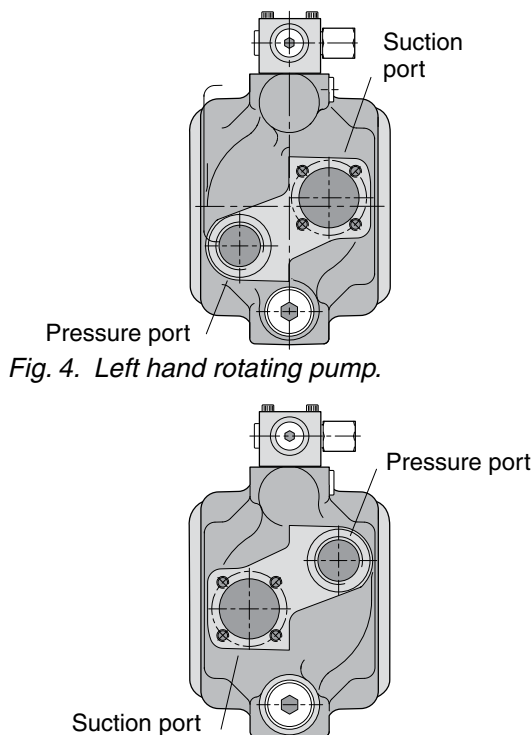
Fig. 5. Right hand rotating pump.
